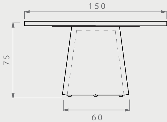
VISTA FRONTAL
