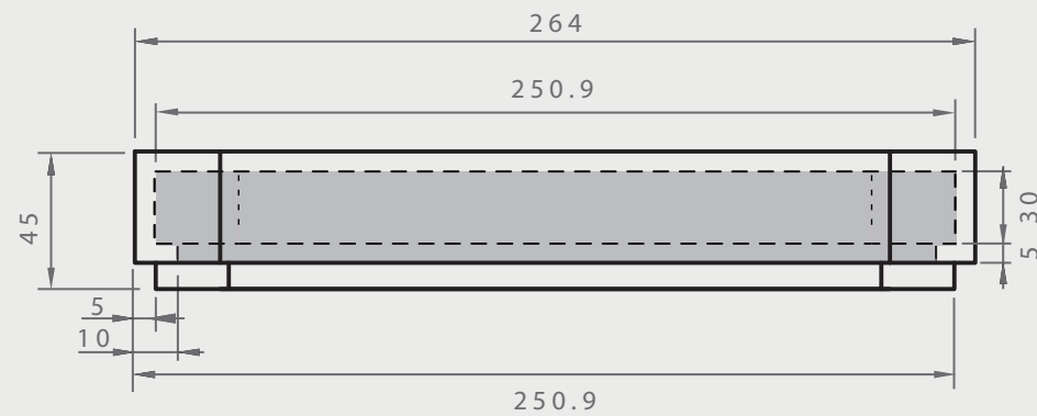
VISTA FRONTAL
