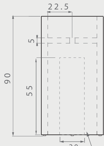
VISTA FRONTAL
