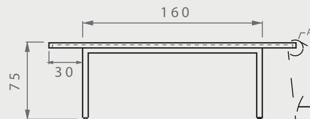
VISTA FRONTAL
